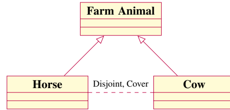
Figure 4: Generalizations
