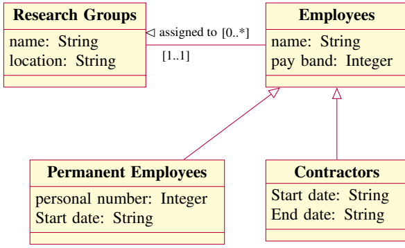
Figure 5: Example 2.1, Diagram \mathcal{D}
