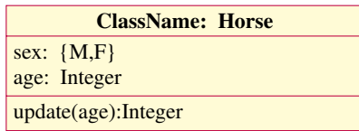
Figure 1: UML class
