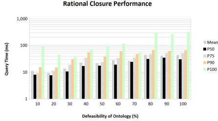
Fig. 3: DIP rational closure performance
