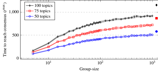
Figure 11: Time to reach consensus for different group sizes. The bands indicate 1\text{-}\sigma , n=10 . The solid symbols on the far right indicate maximum consensus time as N \rightarrow \infty as given by (27).
