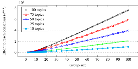
Figure 10: Effort to reach consensus for different group sizes. The bands indicate 1\text{-}\sigma , n=20 .
